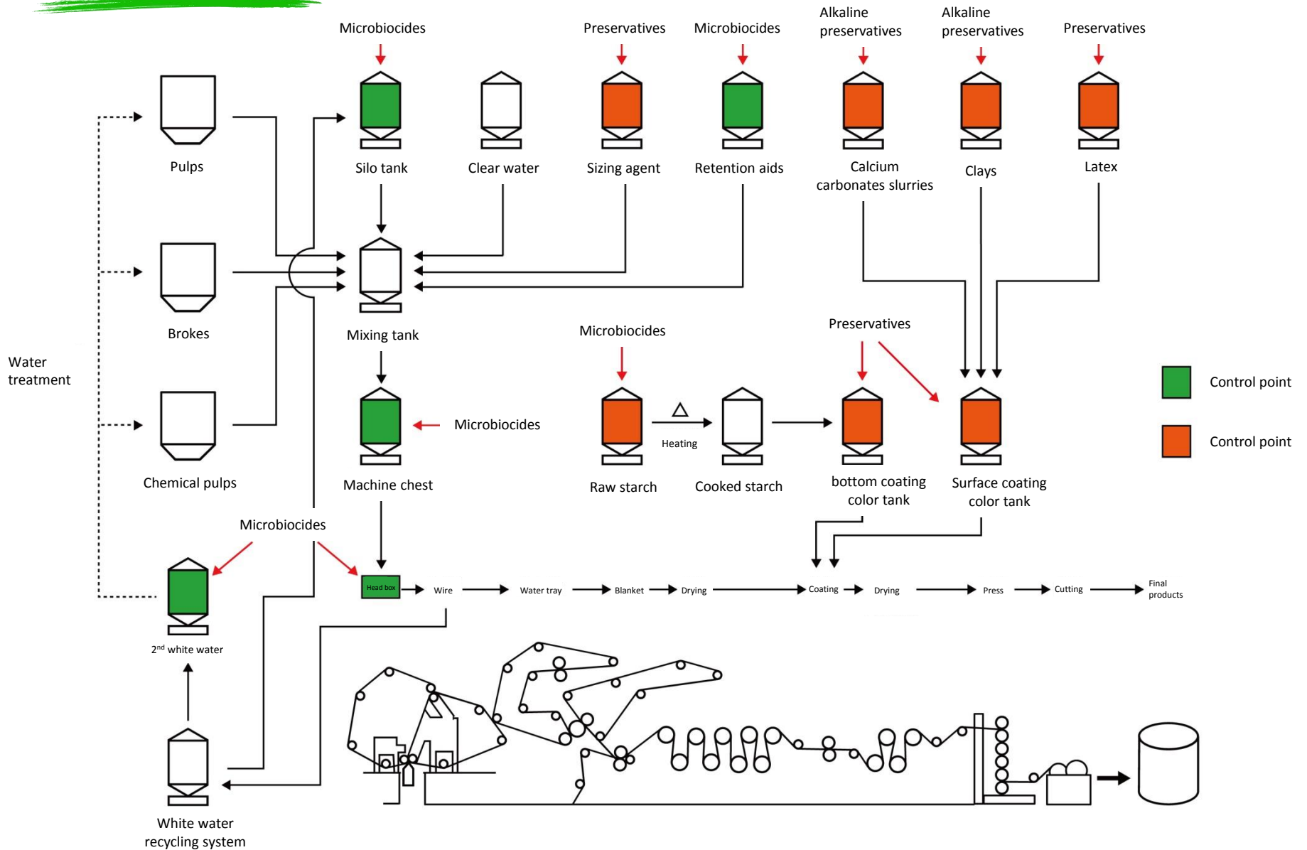
Microbial control diagram for white board paper
