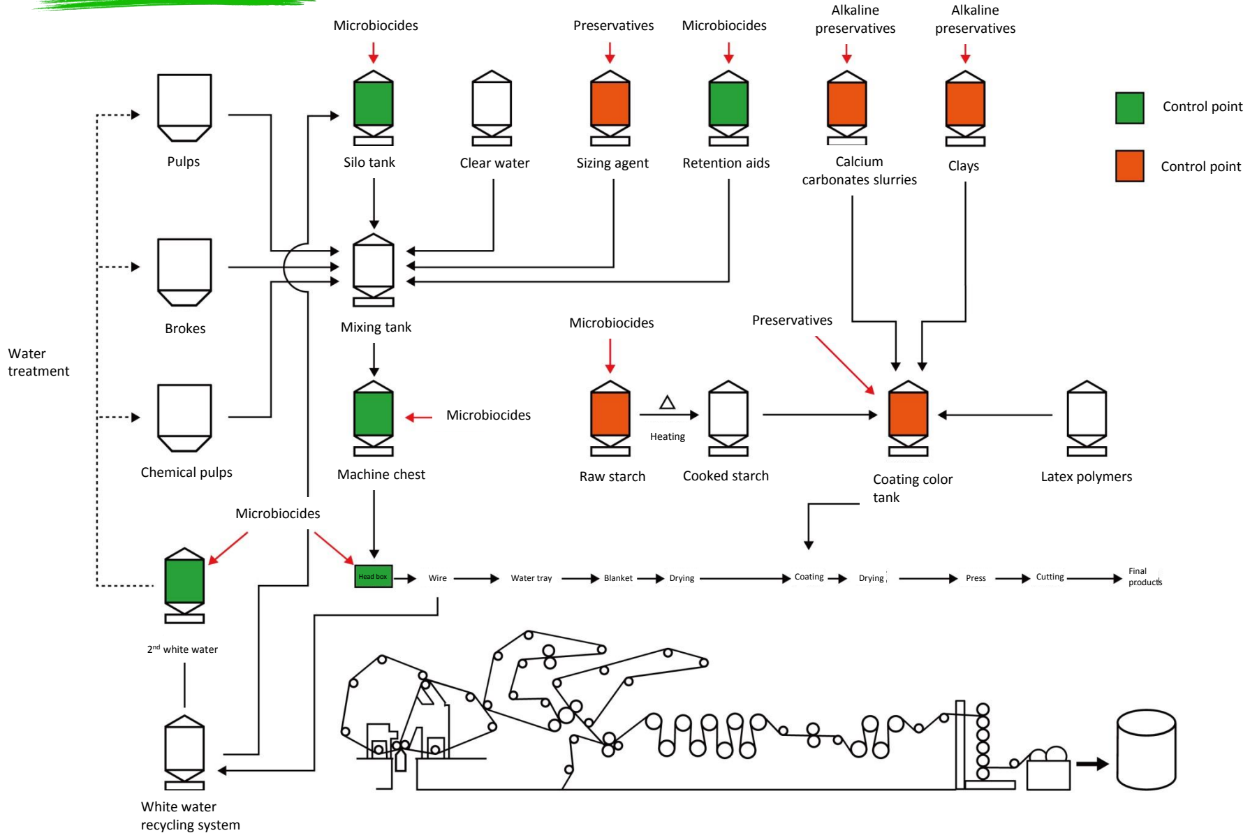
Microbial control diagram for cultural paper
